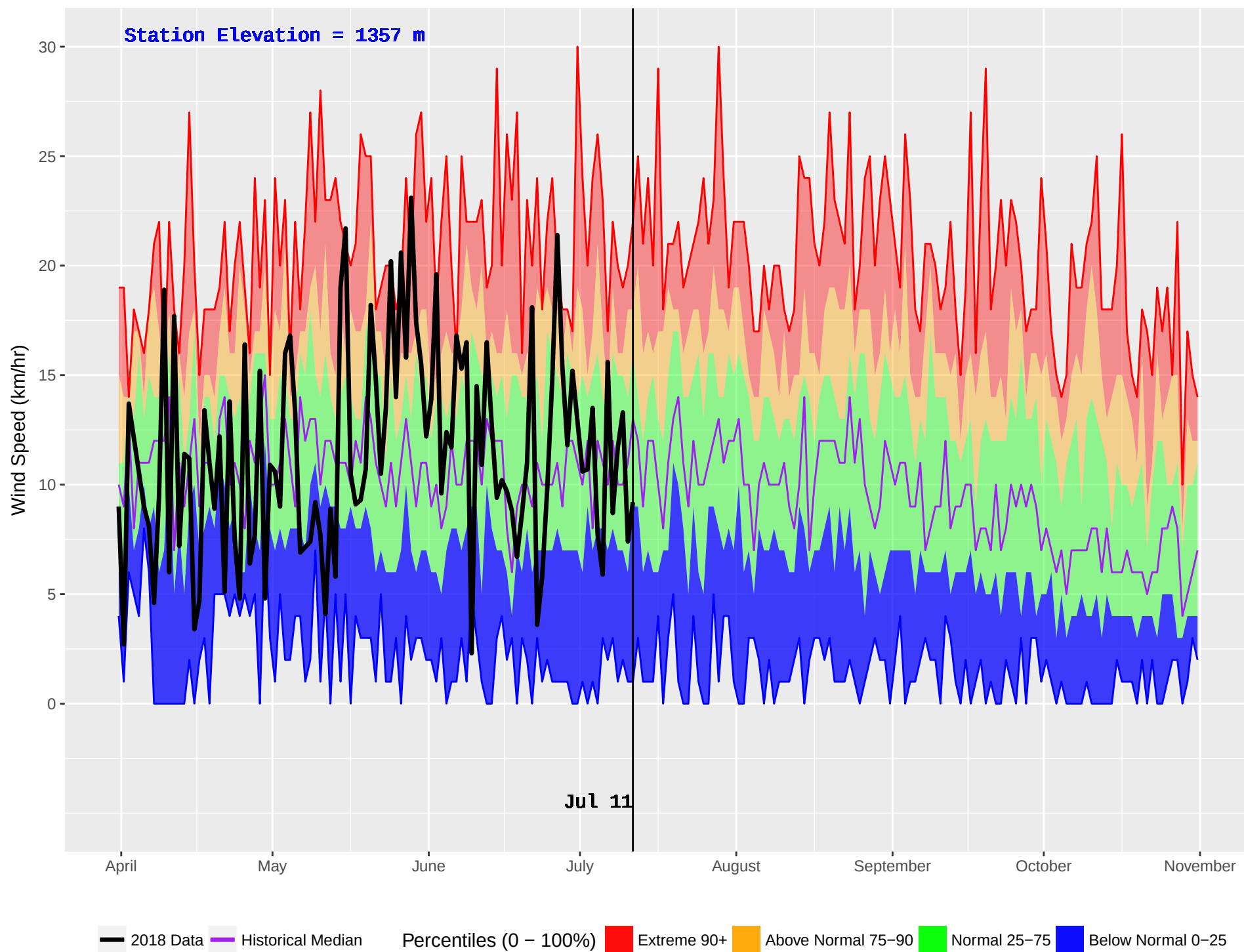
WHITE RIVER (790) : Historical (1989–2016) and Current (2018) Noon Wind Speed
