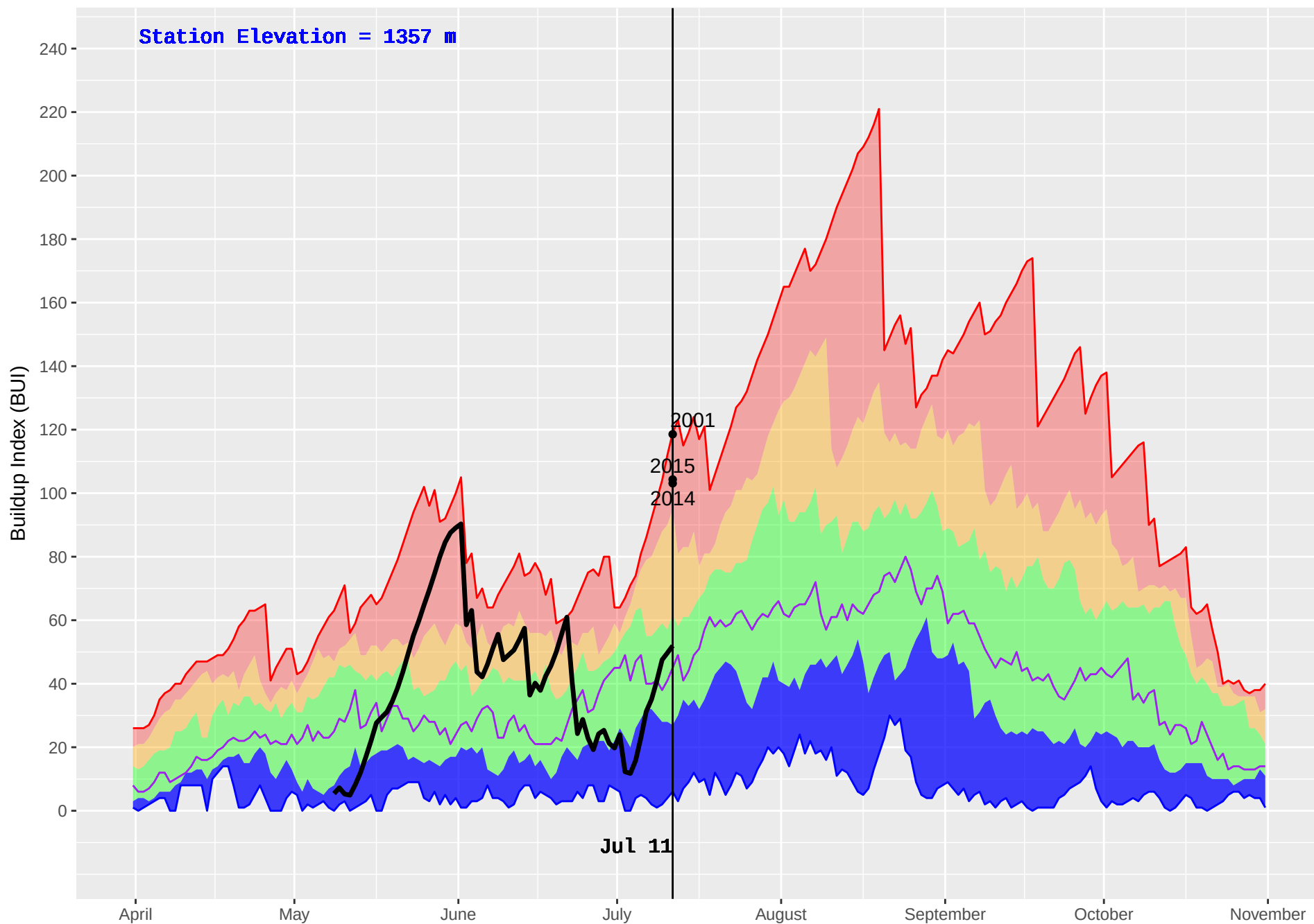
WHITE RIVER (790) : Historical (1989–2016) and Current (2018) Noon Buildup Index (BUI)
