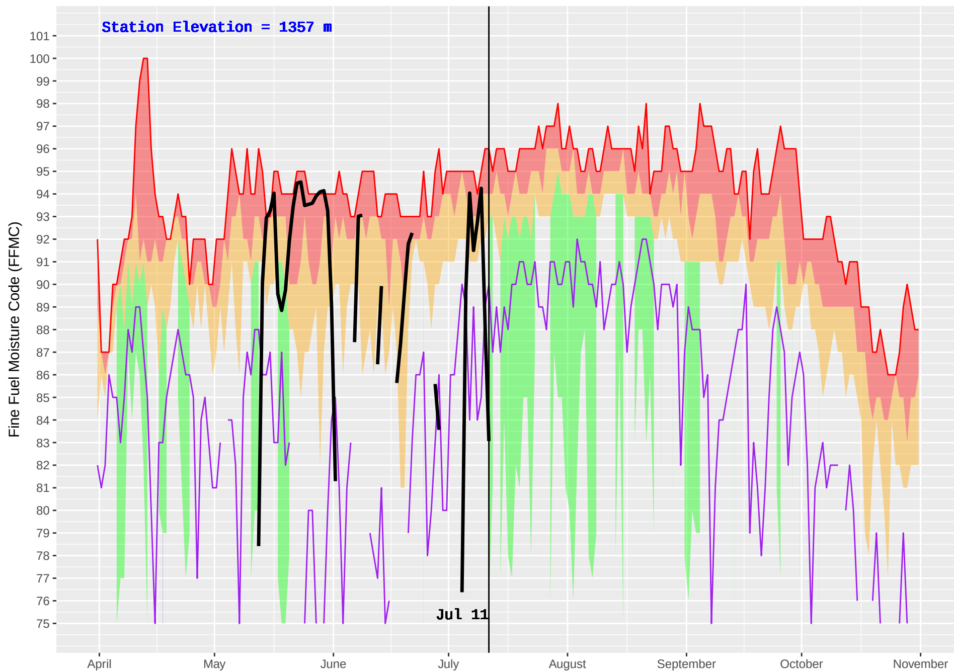
WHITE RIVER (790) : Historical (1989–2016) and Current (2018) Noon Fine Fuel Moisture Code (FFMC)
