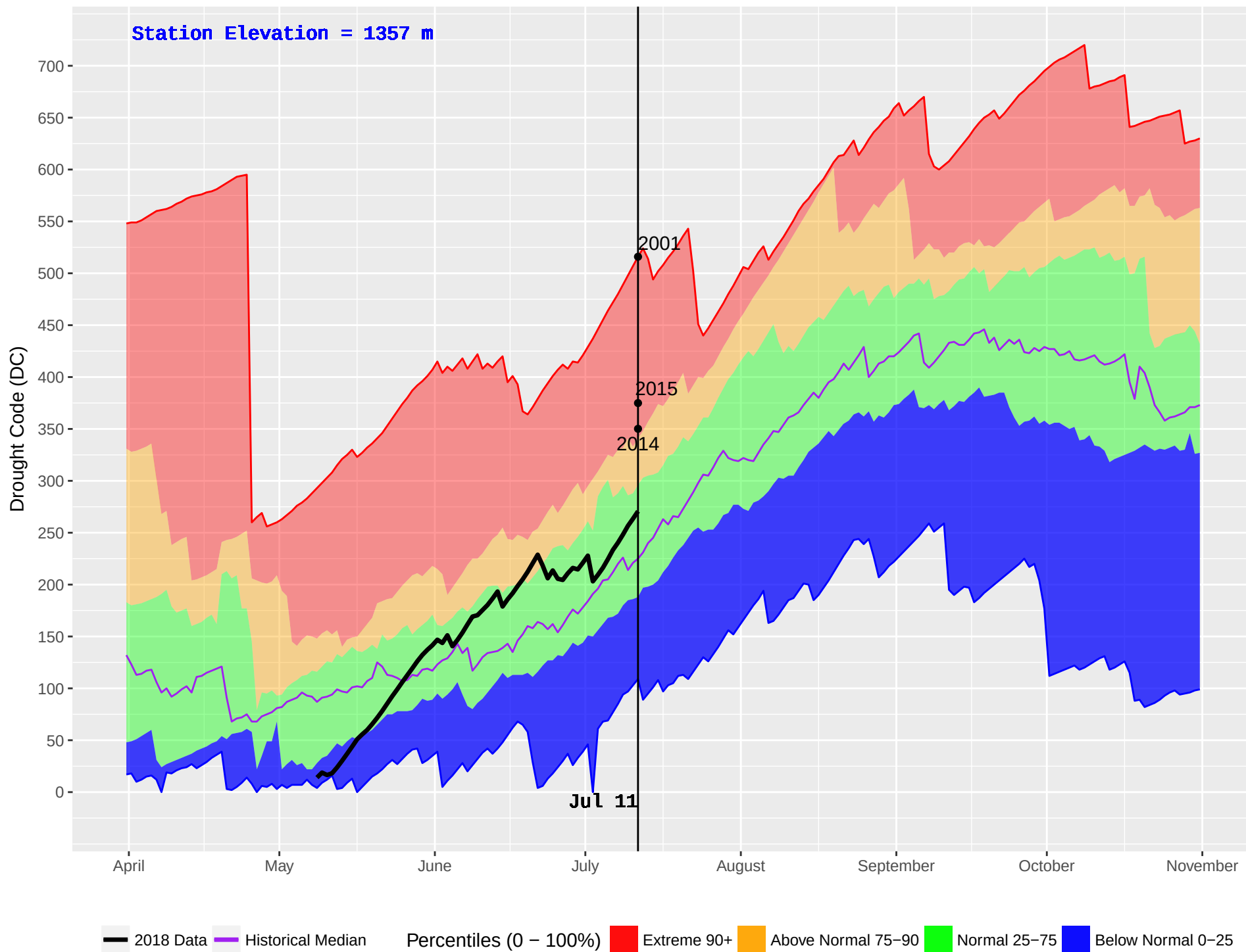
WHITE RIVER (790) : Historical (1989–2016) and Current (2018) Noon Drought Code (DC)
