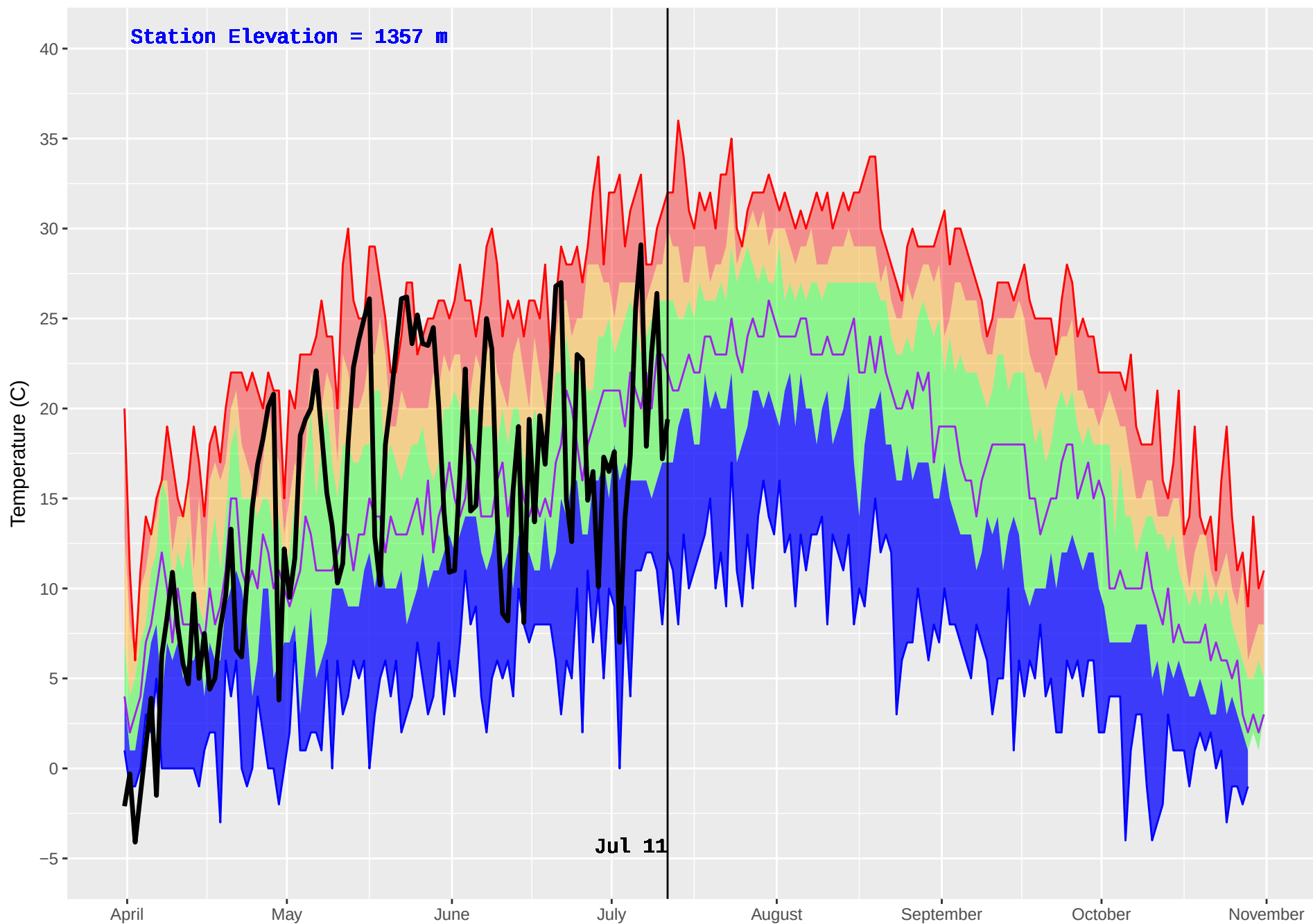
WHITE RIVER (790) : Historical (1989–2016) and Current (2018) Noon Temperature
