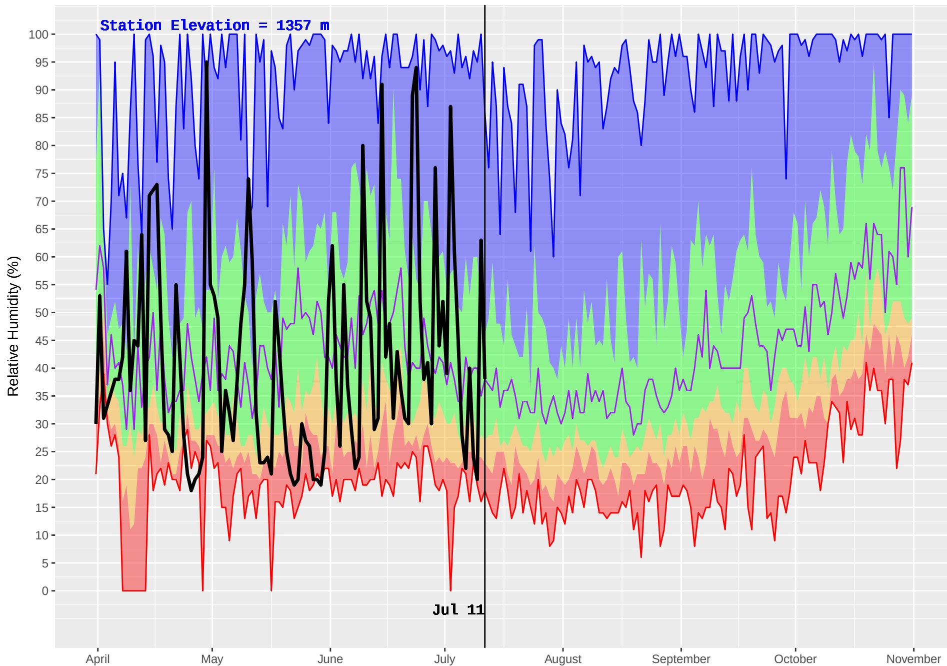
WHITE RIVER (790) : Historical (1989–2016) and Current (2018) Noon Relative Humidity
