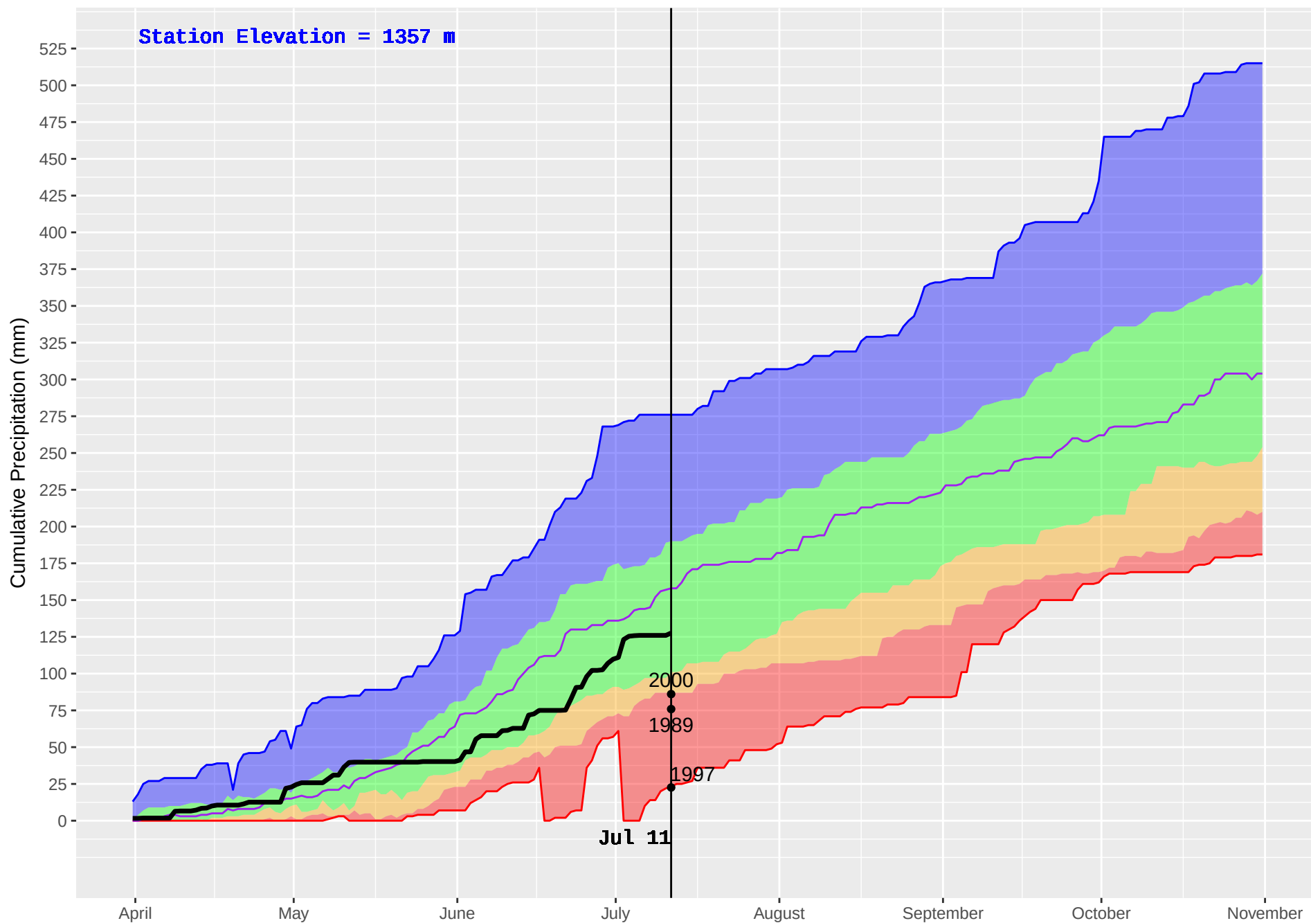
WHITE RIVER (790) : Historical (1989–2016) and Current (2018) Noon Cumulative Precipitation
