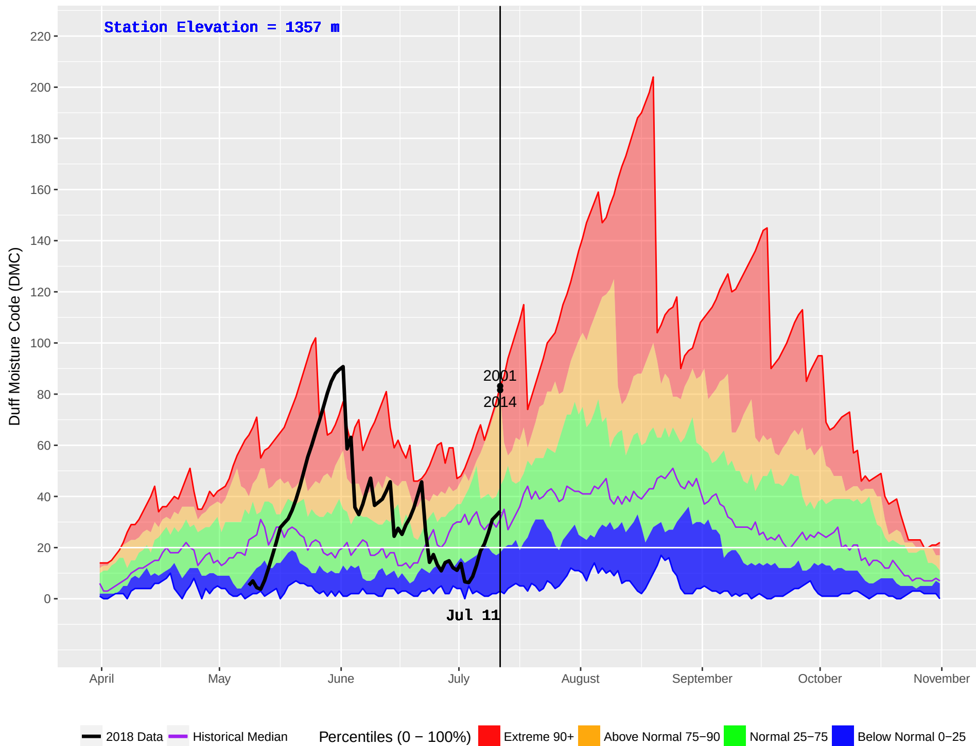
WHITE RIVER (790) : Historical (1989–2016) and Current (2018) Noon Duff Moisture Code (DMC)
